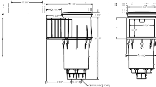
ADMIRAL S20 SKIMMER FOR CONCRETE
